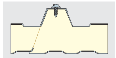
Standard panel joint
