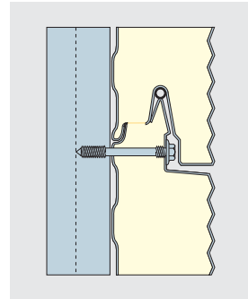
Standard panel joint
