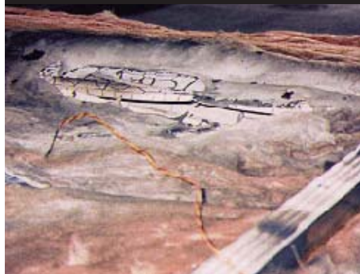
Reduction to vitrified glass (850°C) and total loss of quilt and breather membrane at open overlap joint
