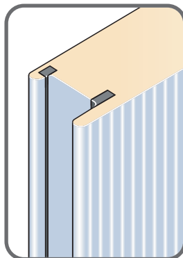
Internal: Simpler typical T&G Joint
