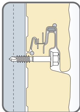
External: Typical engineered joint
